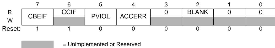
Figure 3-7 EEPROM Status Register (ESTAT)
