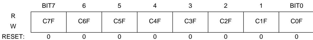
Figure 3-12 Main Timer Interrupt Flag 1 (TFLG1)
