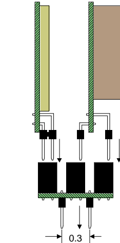
Example E AD11BP2-SB plugs 2 boards into a solderless breadboard at once
